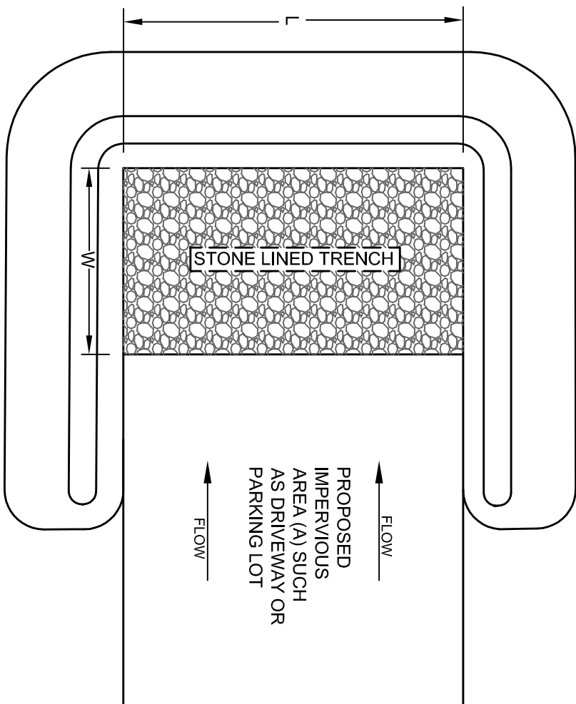
Plan view
